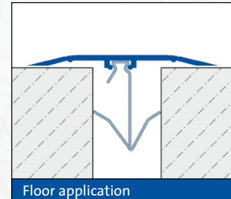
Floor application
